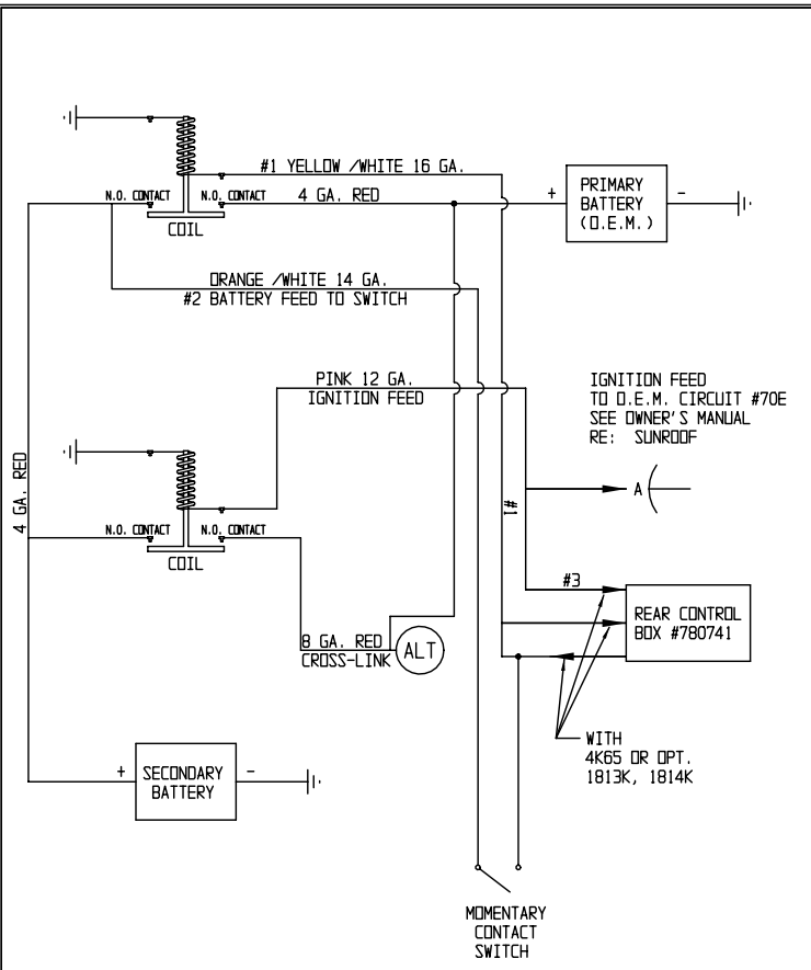
SCHEMATIC - DUAL BATTERIES 1997 - 1999 "K" & "CK" MODEL LIMOUSINES
